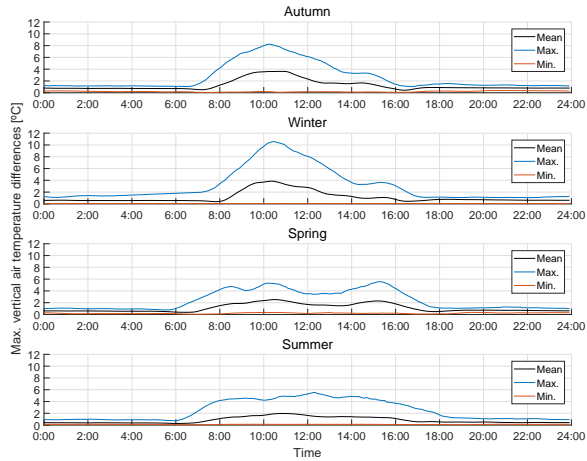
Figure 17: Maximum vertical air temperatures differences.
