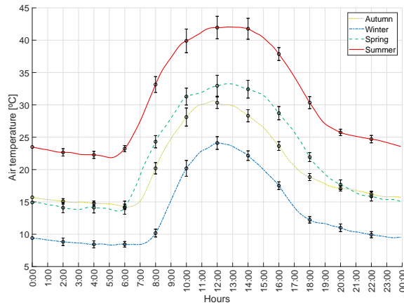
Figure 4: Average day and confident intervals ( \pm 1\sigma ) of mean air temperature per season.
