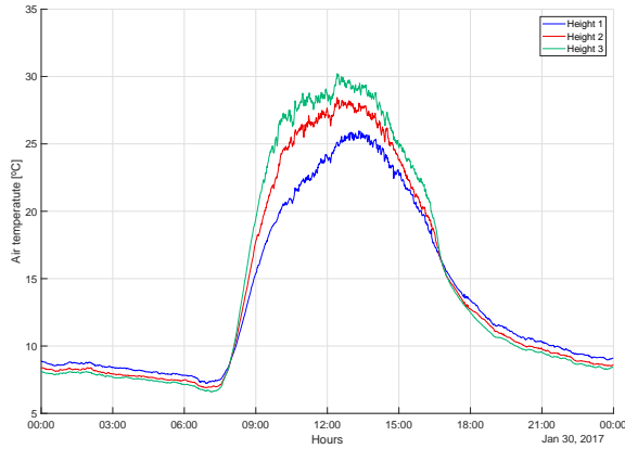
Figure 3: Mean air temperature for each height on January, 30th 2017.
