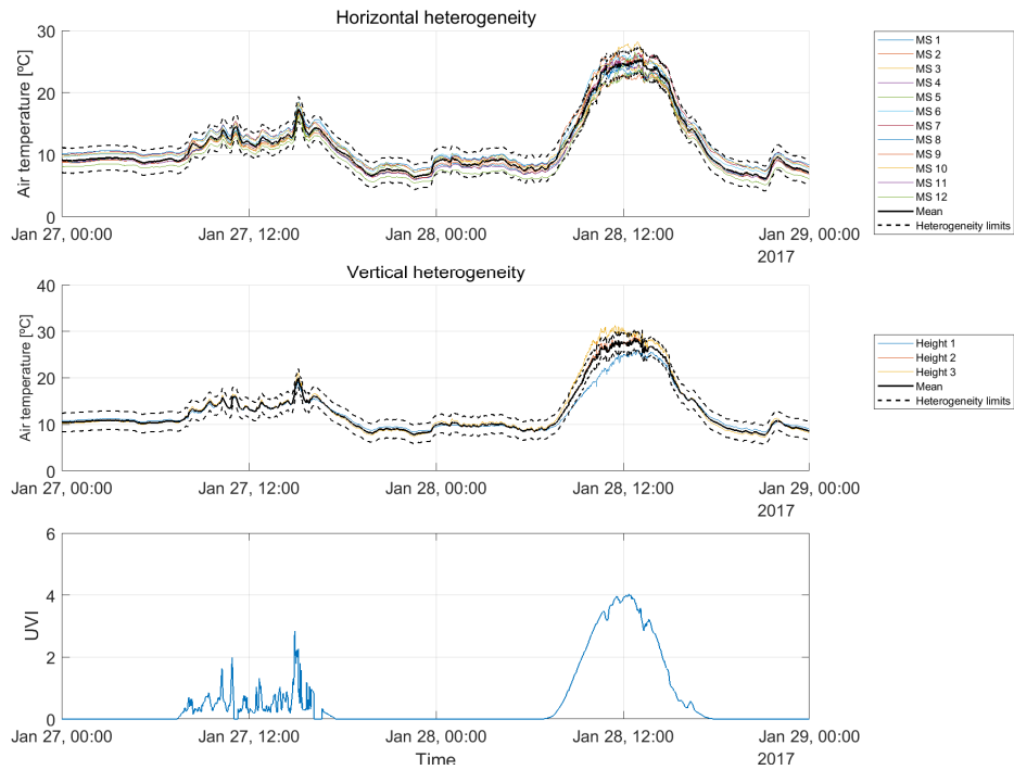
Figure 11: Horizontal heterogeneity, vertical heterogeneity and UVI for two consecutive days (January, 27th and 28th 2017), the first one cloudy and the second one sunny.
