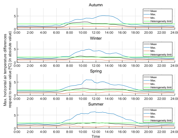
Figure 14: Maximum horizontal air temperatures differences respect to mean value, in absolute value.
