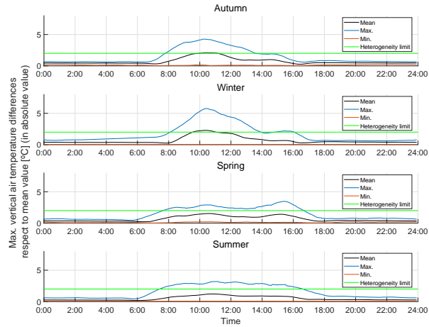
Figure 15: Maximum vertical air temperatures differences respect to mean value, in absolute value.
