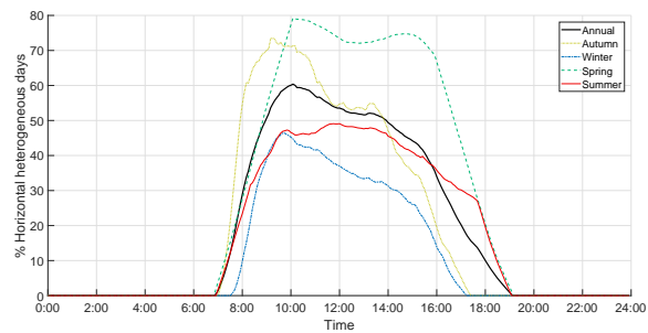
Figure 12: Percentage of horizontal heterogeneous days at every moment of time throughout the day.
