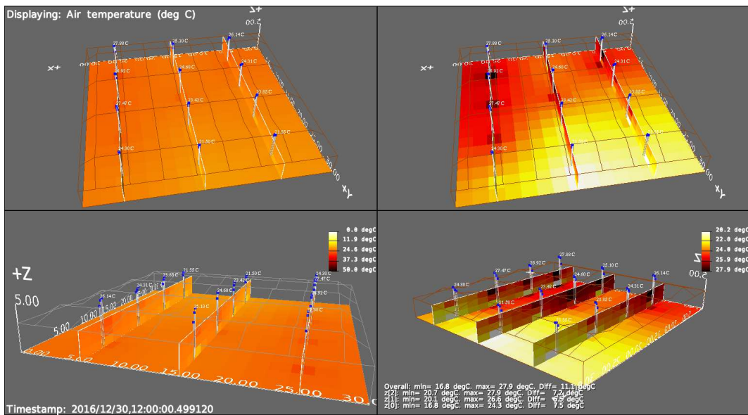
Figure 5: Air temperature distribution inside the greenhouse (four different views). Image capture of the 3D video at 12:00, 30th Dec 2016.
