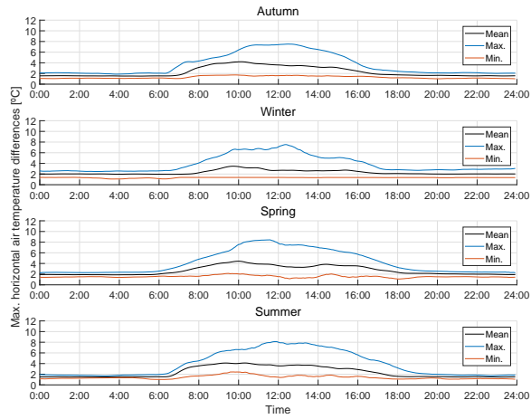
Figure 16: Maximum horizontal air temperatures differences.
