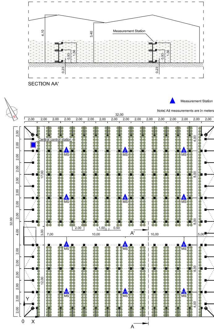
Figure 1: Drawing of the greenhouse, where also are defined the locations of the measurement stations.
