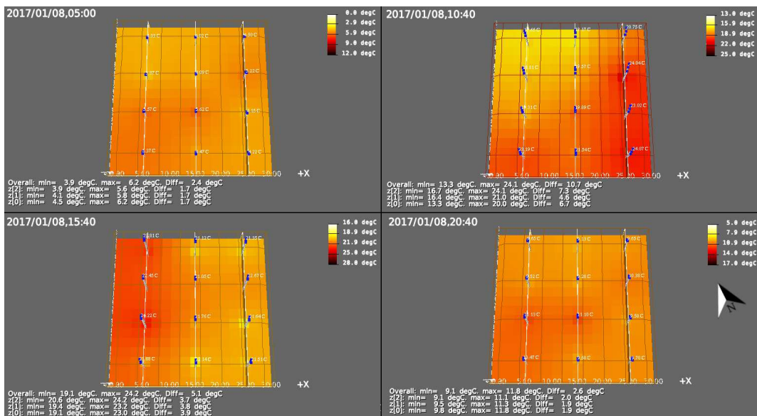
Figure 6: Air temperature distribution inside the greenhouse at four different moments along the a day: 5:00 a.m, 10:40 a.m, 15:40 a.m and 20:40 a.m.
